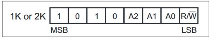
Figure 7-1. Device Address
